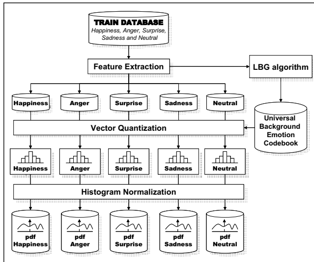
Figure 1: Emotion model generation procedure
